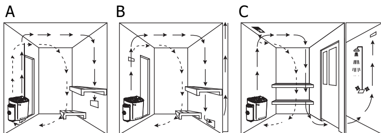
Fig. 7 Air ventilation
